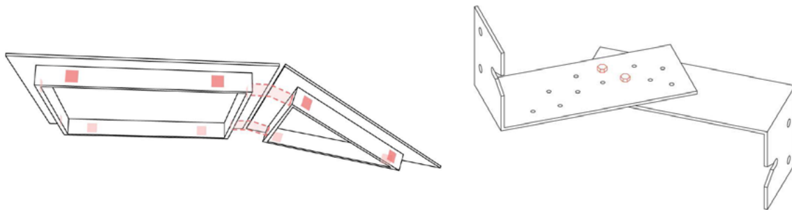
Figure 2: The polygonal elements consist of a thin plate material to which vertical ribs are added parallel to the edges to generate stiffness. Two connection points are located on each rib to join adjacent elements. Elements are joined with identical connectors which can accommodate multiple angles.
